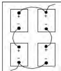
Figure 3 Voltage/Capacity Increase
